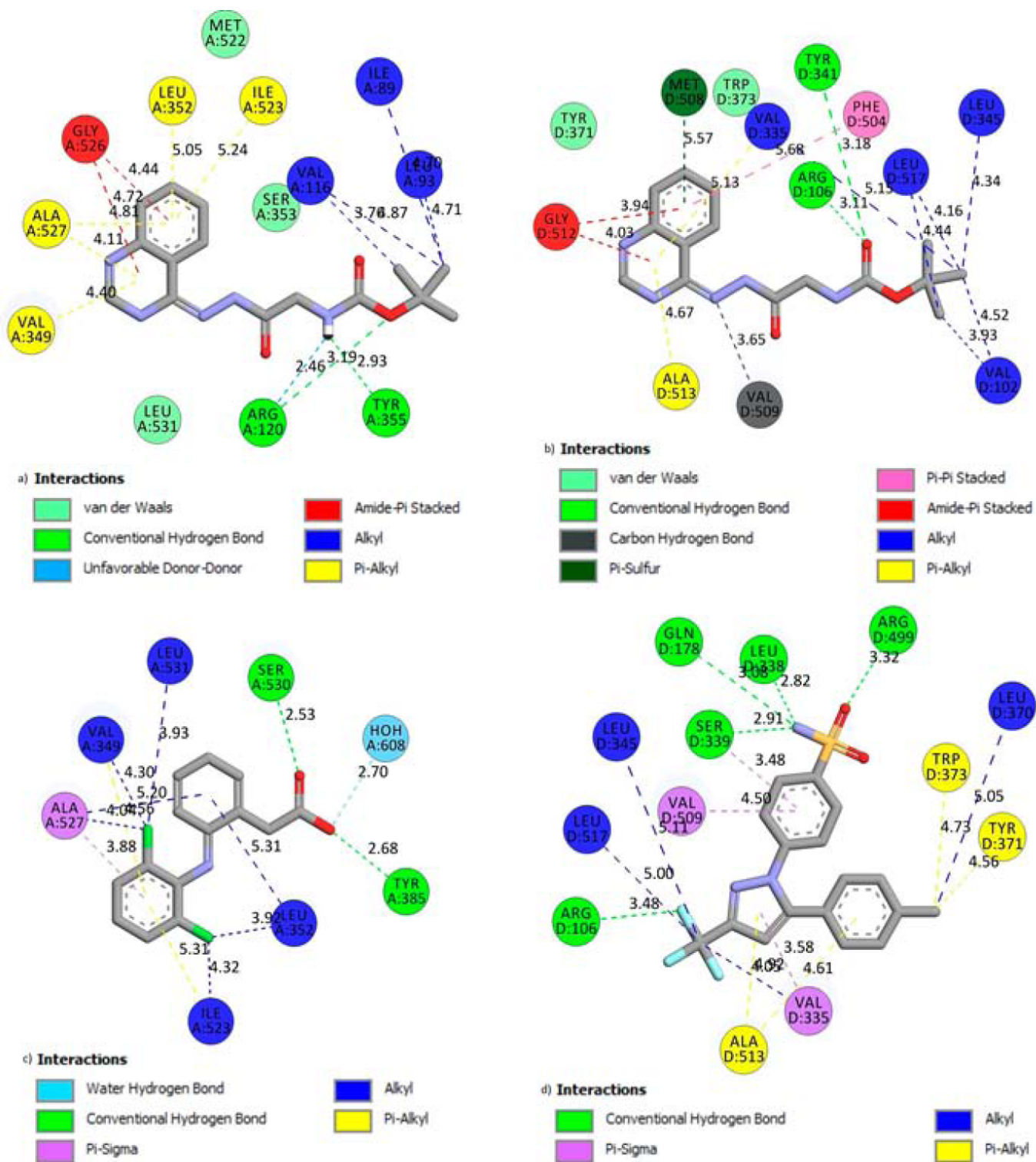
Fig. (1). Visualization of affinity according to the docking a) compound 1.13 with COX-1; b) compound 1.13 with COX-2; c) Diclofenac with COX-1; d) Celecoxib with COX-2.
