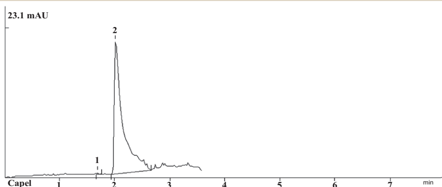
Fig. 1. Electrophoregram of the solution of SS of chlorhexidine (peak 2 – chlorhexidine).
