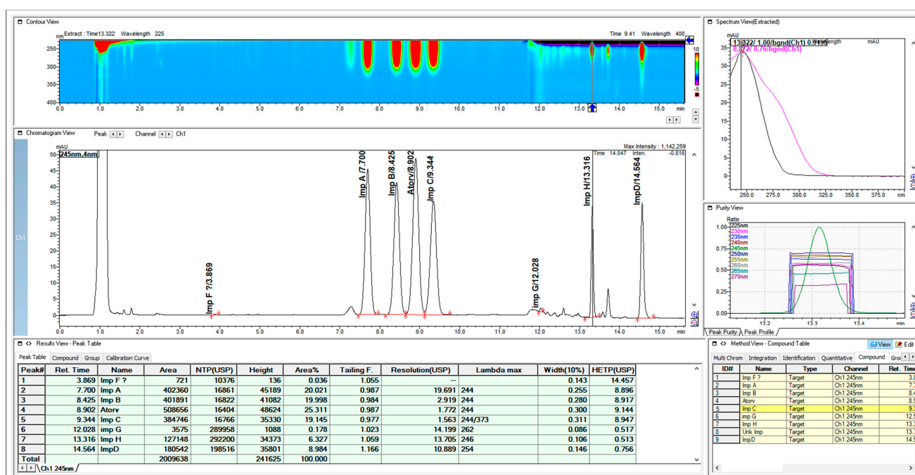
Figure 6. Separation of atorvastatin and its impurities using Poroshell C18ec 100 mm x 4.6 mm, 2.7 μm, with 3 μl injection volume.
