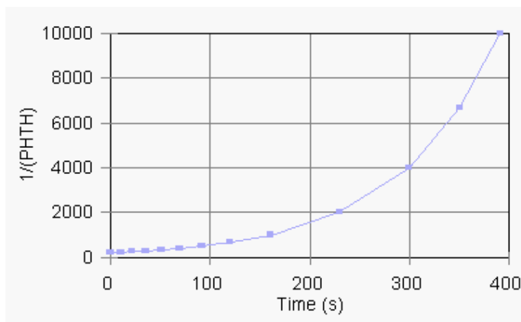
Figure 2. A plot of the reciprocal of the concentration of phenolphthalein versus time for the reaction between phenolphthalein and excess \text{OH}^- ion is not a straight line, which shows that this reaction is not second order in phenolphthalein.
