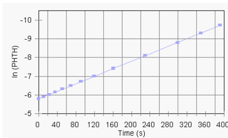
Figure 1. A plot of the natural log of the concentration of phenolphthalein versus time for the reaction between phenolphthalein and excess \text{OH}^- ion is a straight line, which shows that this reaction is first order in phenolphthalein.
