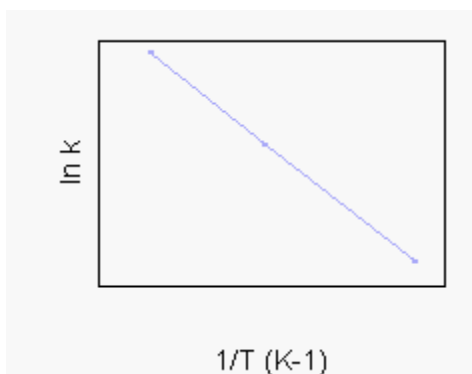
Figure 1. A plot of the natural log of the rate constant for the reaction at different temperatures versus the inverse of the temperature in kelvin is a straight line with a slope equal to -E_a/R .
